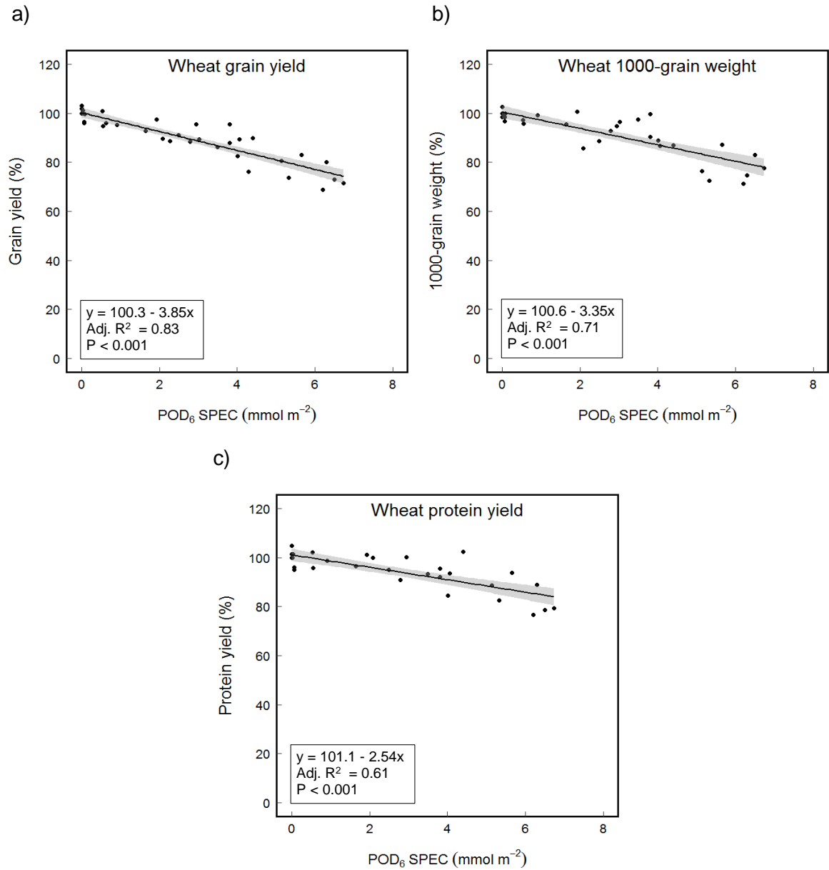
Figure III.10: The relationship between the percentage yield of wheat and stomatal O_3 flux ( POD_6 SPEC) for the wheat flag leaf based on five wheat cultivars from three or four European countries (Belgium, Finland, Italy, Sweden): a) grain yield, b) 1000-grain weight, and c) protein yield. The grey area indicates the 95%-confidence interval (Grünhage et al., 2012).
