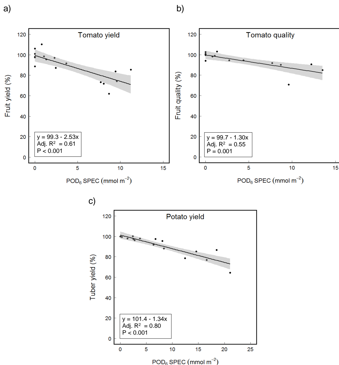
Figure III.11: The relationship between the percentage a) tomato fruit yield and b) tomato fruit quality and POD_6\ SPEC for sunlit leaves (González-Fernández et al., 2014) based on data from Italy and Spain, and c) tuber yield of potato and POD_6\ SPEC for sunlit leaves (Pleijel et al., 2007) based on data from Belgium, Finland, Germany, Sweden. The grey area indicates the 95%-confidence interval.
