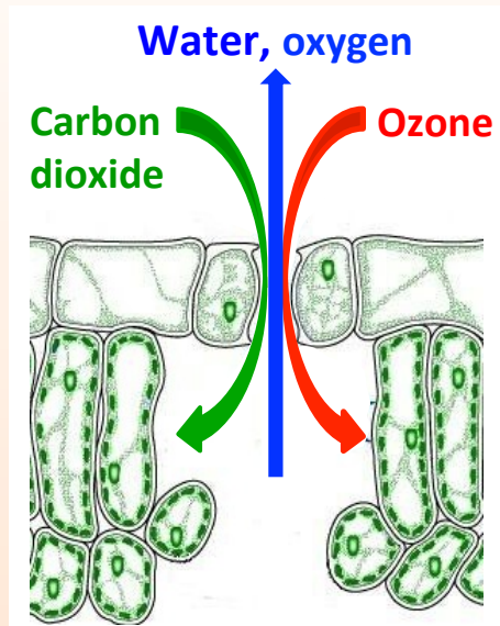
A schematic showing a cross section through a leaf. Arrows show the uptake of carbon dioxide and ozone, and the release of water and oxygen through leaf pores.
