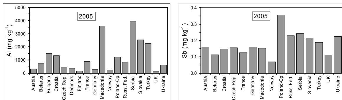
Figure 3.22. Median aluminium (left) and antimony (right) concentration in mosses per country in 2005.
