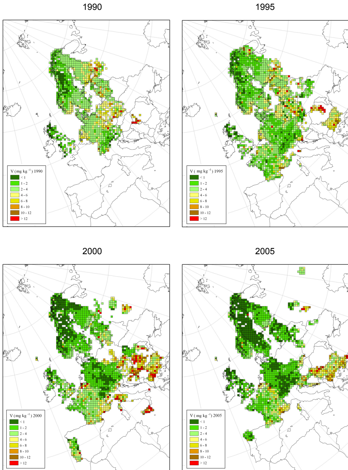
Figure 3.17. Mean concentration of vanadium in mosses per EMEP grid square in 1990, 1995, 2000 and 2005.
