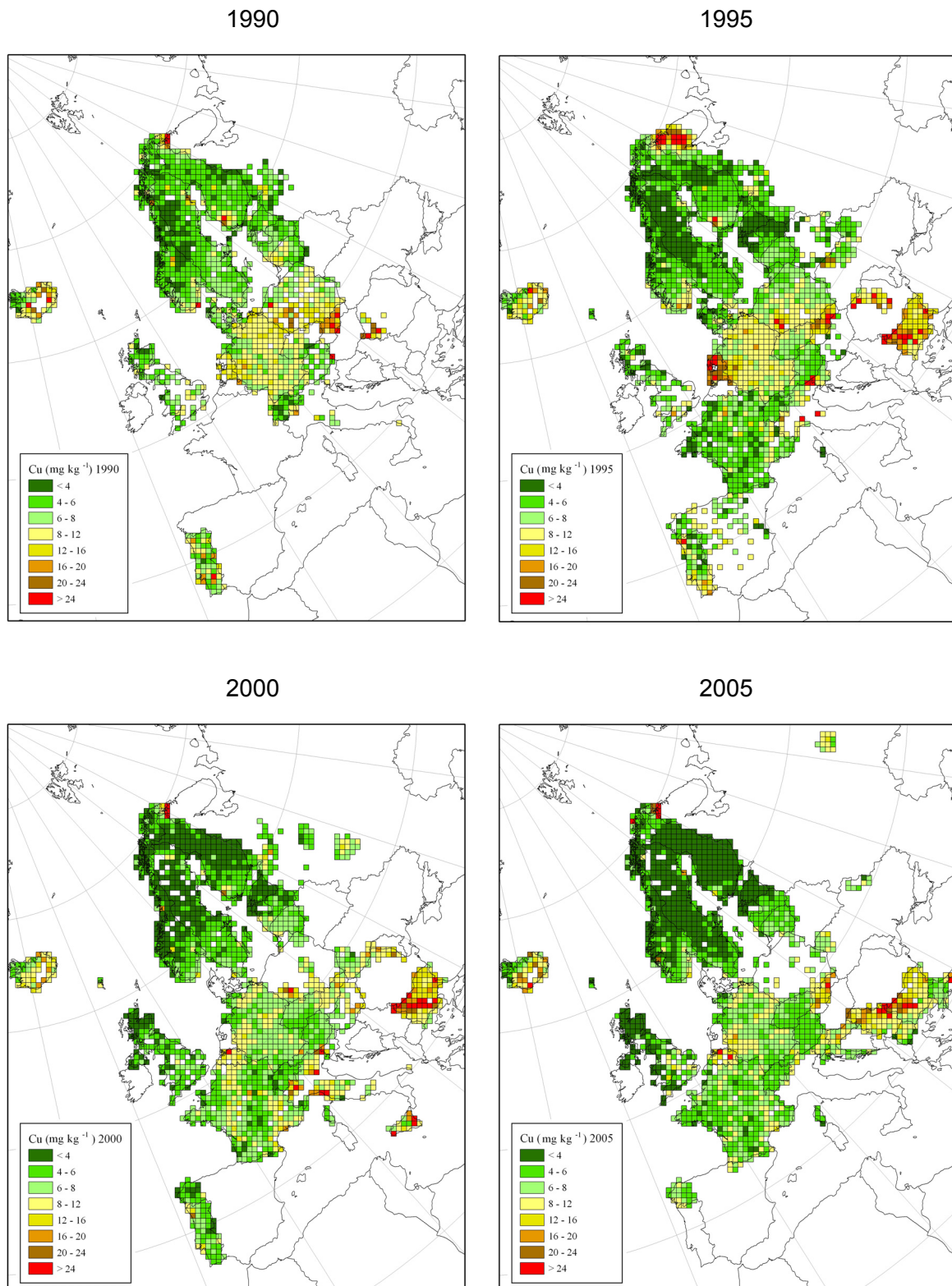
Figure 3.7. Mean concentration of copper in mosses per EMEP grid square in 1990, 1995, 2000 and 2005.
