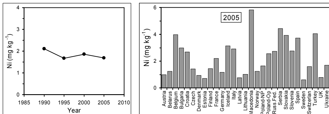
Figure 3.16. Average of median nickel concentration in mosses for countries (n = 16) that reported nickel data in all survey years (left) and median nickel concentration in mosses per country in 2005 (right).
