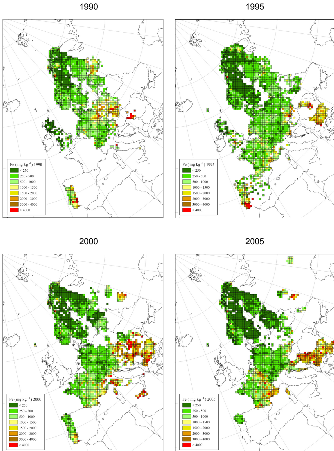
Figure 3.9. Mean concentration of iron in mosses per EMEP grid square in 1990, 1995, 2000 and 2005.
