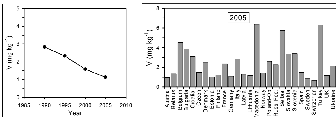
Figure 3.18. Average of median vanadium concentration in mosses for countries (n = 11) that reported vanadium data in all survey years (left) and median vanadium concentration in mosses per country in 2005 (right).
