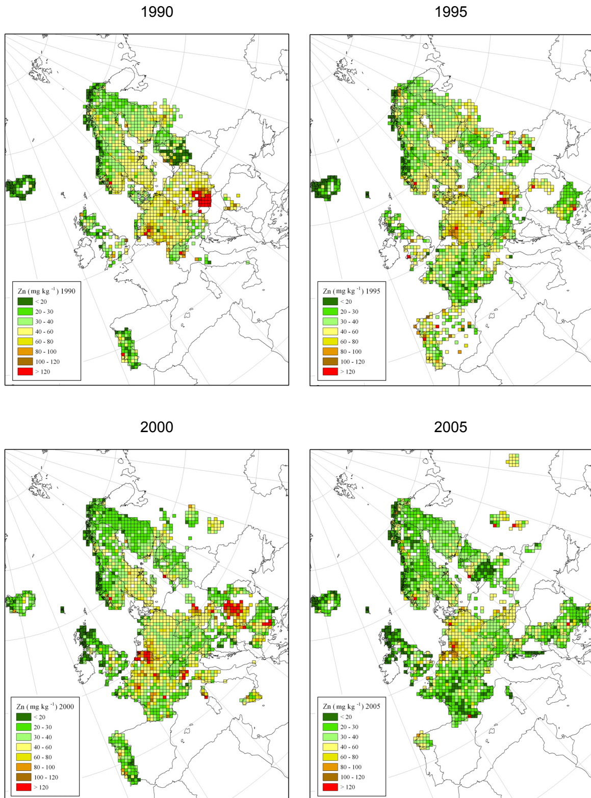
Figure 3.19. Mean concentration of zinc in mosses per EMEP grid square in 1990, 1995, 2000 and 2005.
