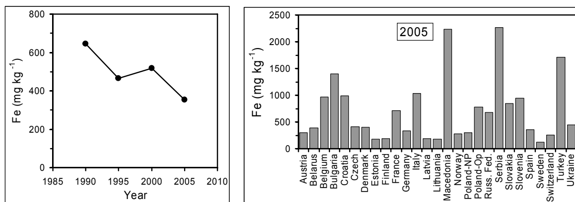
Figure 3.10. Average of median iron concentration in mosses for countries (n = 13) that reported iron data in all survey years (left) and median iron concentration in mosses per country in 2005 (right).
