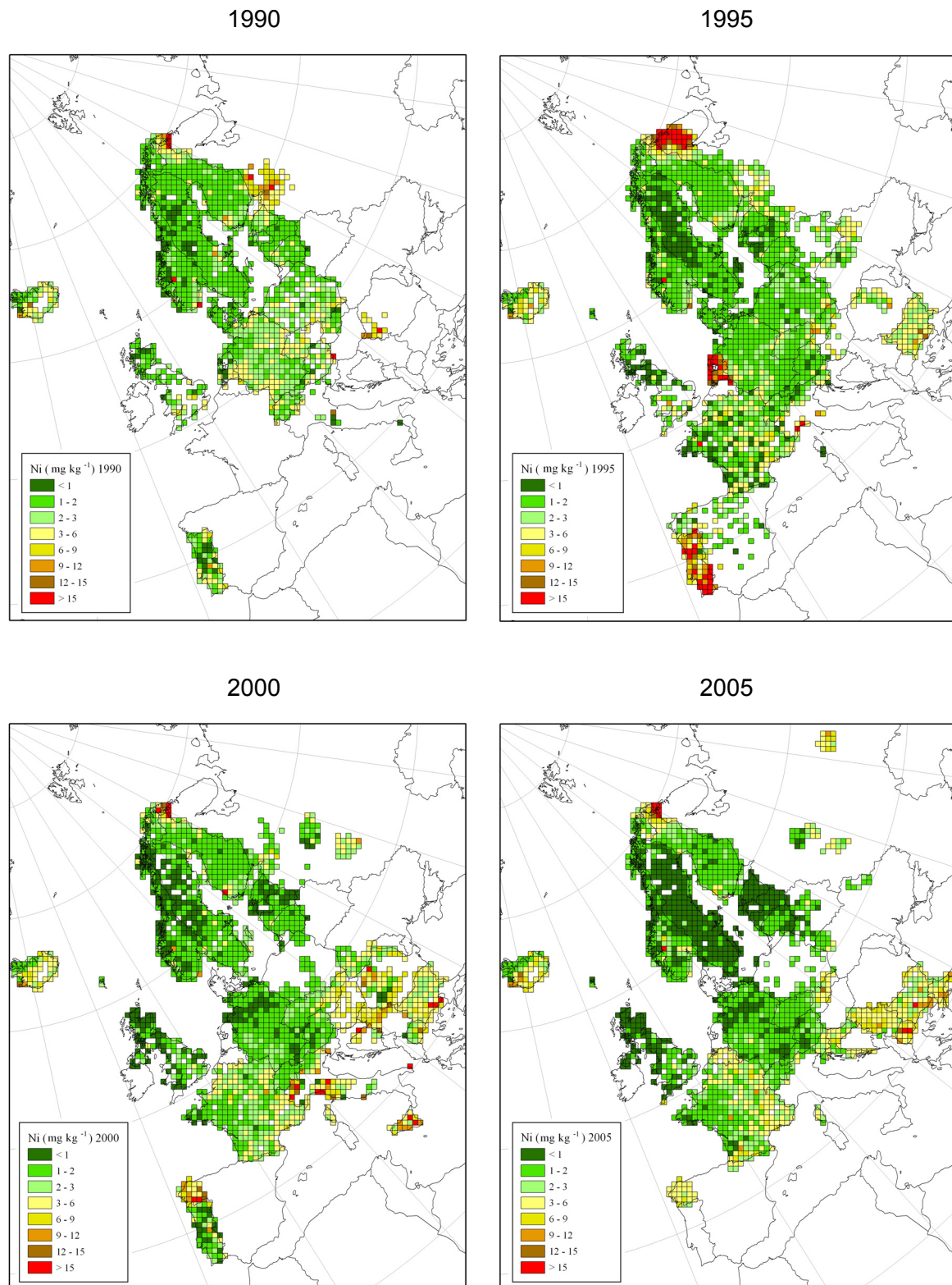
Figure 3.15. Mean concentration of nickel in mosses per EMEP grid square in 1990, 1995, 2000 and 2005.
