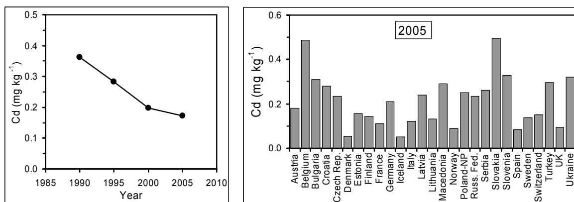
Figure 3.4. Average of median cadmium concentration in mosses for countries (n = 16) that reported cadmium data in all survey years (left) and median cadmium concentration in mosses per country in 2005 (right).
