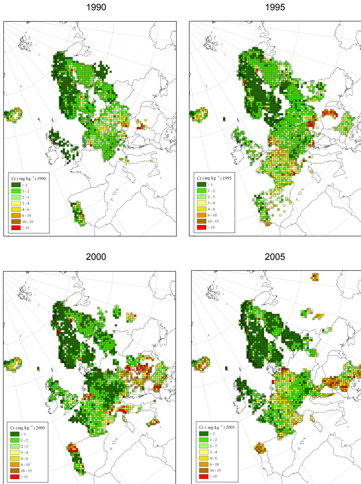
Figure 3.5. Mean concentration of chromium in mosses per EMEP grid square in 1990, 1995, 2000 and 2005.
