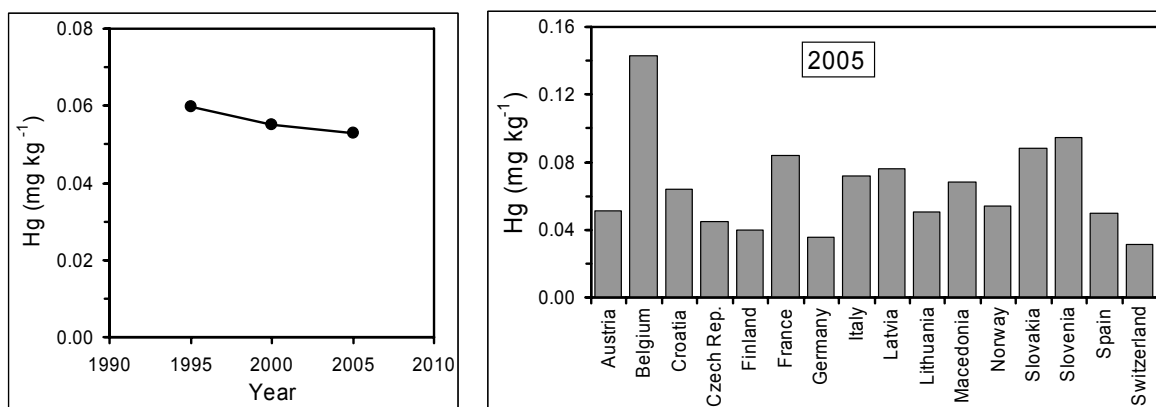
Figure 3.14. Average of median mercury concentration in mosses for countries (n = 8) that reported mercury data in all survey years (left) and median mercury concentration in mosses per country in 2005 (right).
