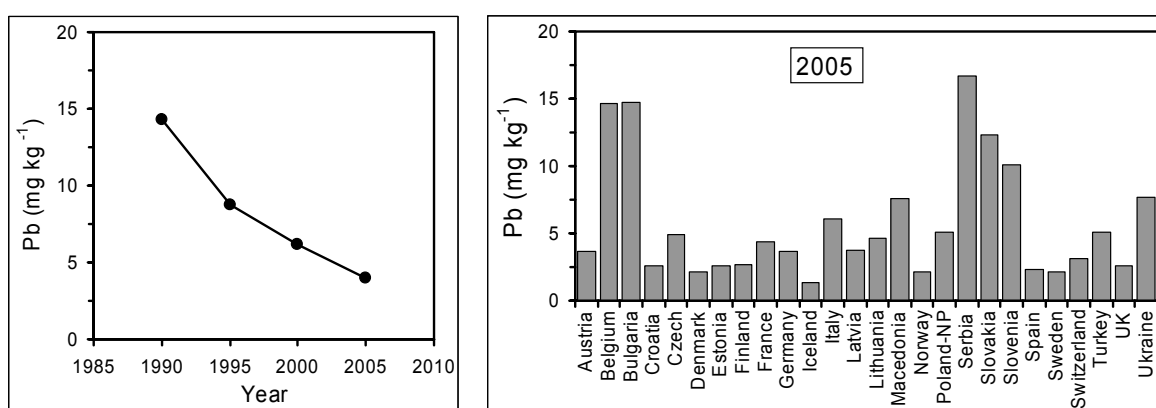
Figure 3.12. Average of median lead concentration in mosses for countries (n = 16) that reported lead data in all survey years (left) and median lead concentration in mosses per country in 2005 (right).
