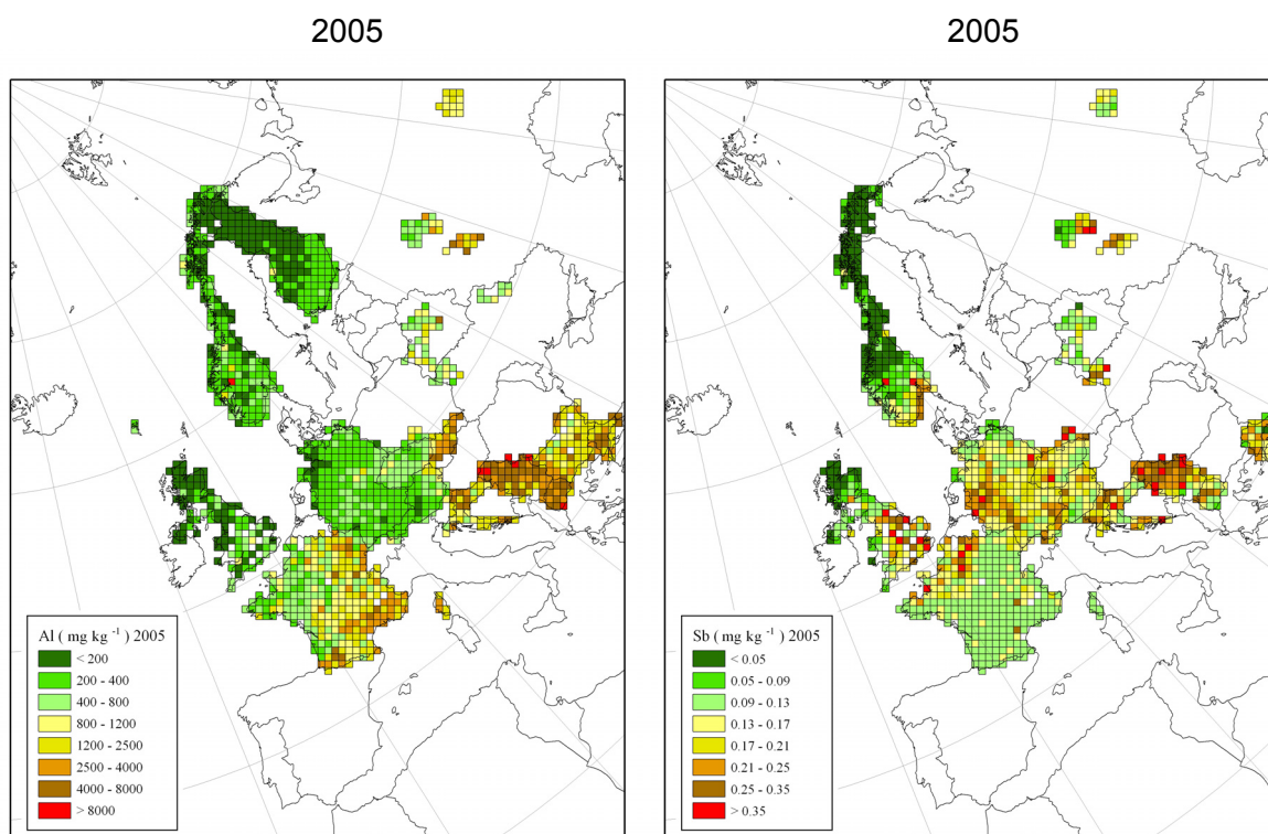
Figure 3.21. Mean concentration of aluminium (left) and antimony (right) in mosses per EMEP grid square in 2005.
