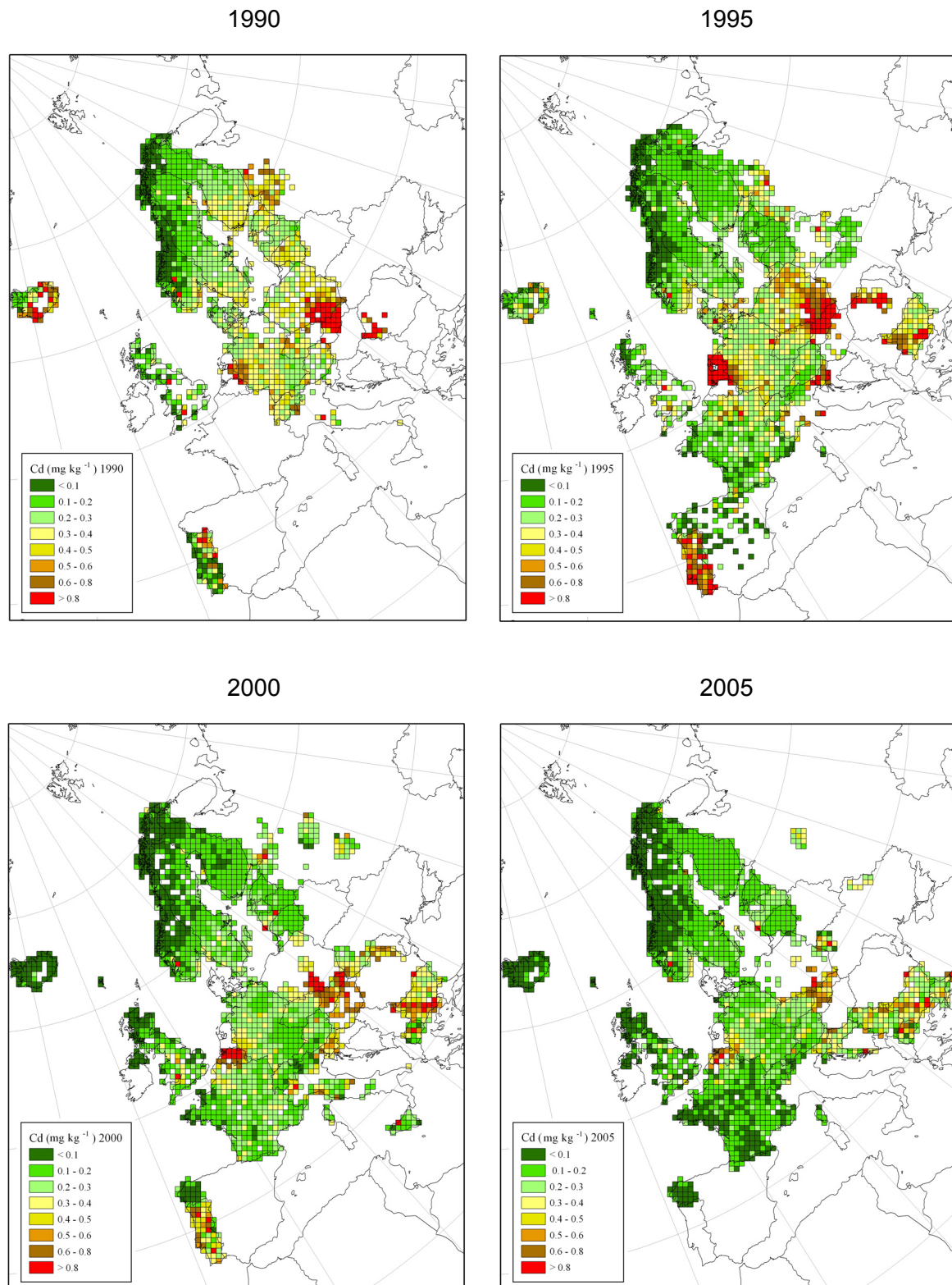
Figure 3.3. Mean concentration of cadmium in mosses per EMEP grid square in 1990, 1995, 2000 and 2005.
