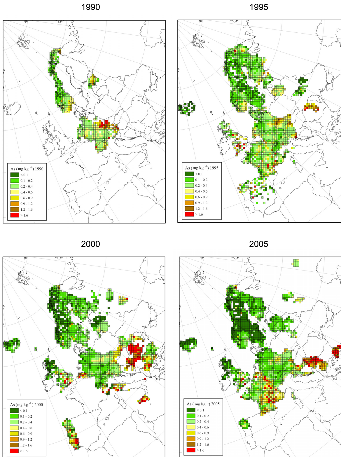
Figure 3.1. Mean concentration of arsenic in mosses per EMEP grid square in 1990, 1995, 2000 and 2005.
