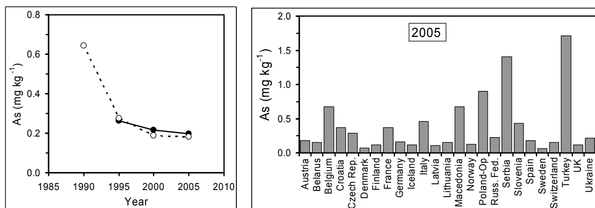
Figure 3.2. Average of median arsenic concentration in mosses for countries (n = 15) that reported arsenic data in 1995, 2000 and 2005, the broken line between 1990 and 2005 is based on data from only five countries (left), and median arsenic concentration in mosses per country in 2005 (right).
