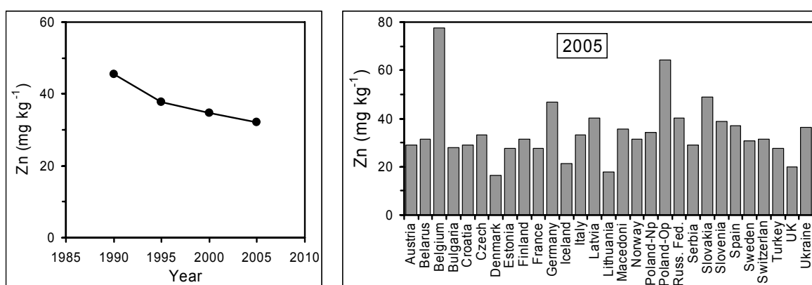
Figure 3.20. Average of median zinc concentration in mosses for countries ( n = 16 ) that reported zinc data in all survey years (left) and median zinc concentration in mosses per country in 2005 (right).
