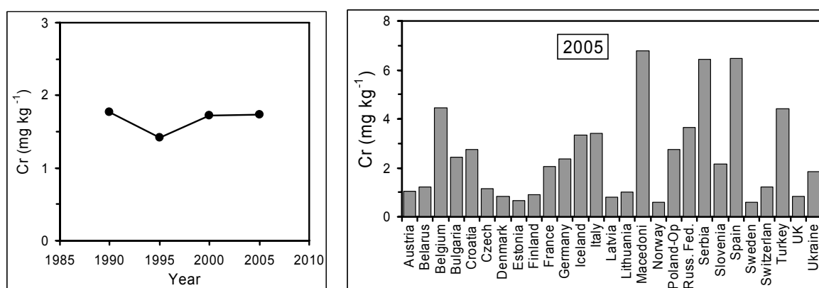
Figure 3.6. Average of median chromium concentration in mosses for countries ( n = 14 ) that reported chromium data in all survey years (left) and median chromium concentration in mosses per country in 2005 (right).
