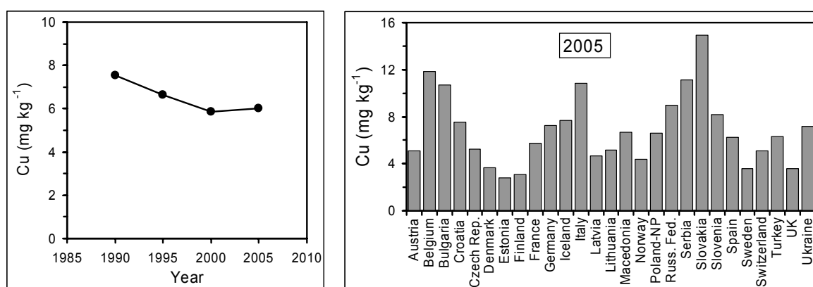
Figure 3.8. Average of median copper concentration in mosses for countries (n = 16) that reported copper data in all survey years (left) and median copper concentration in mosses per country in 2005 (right).
