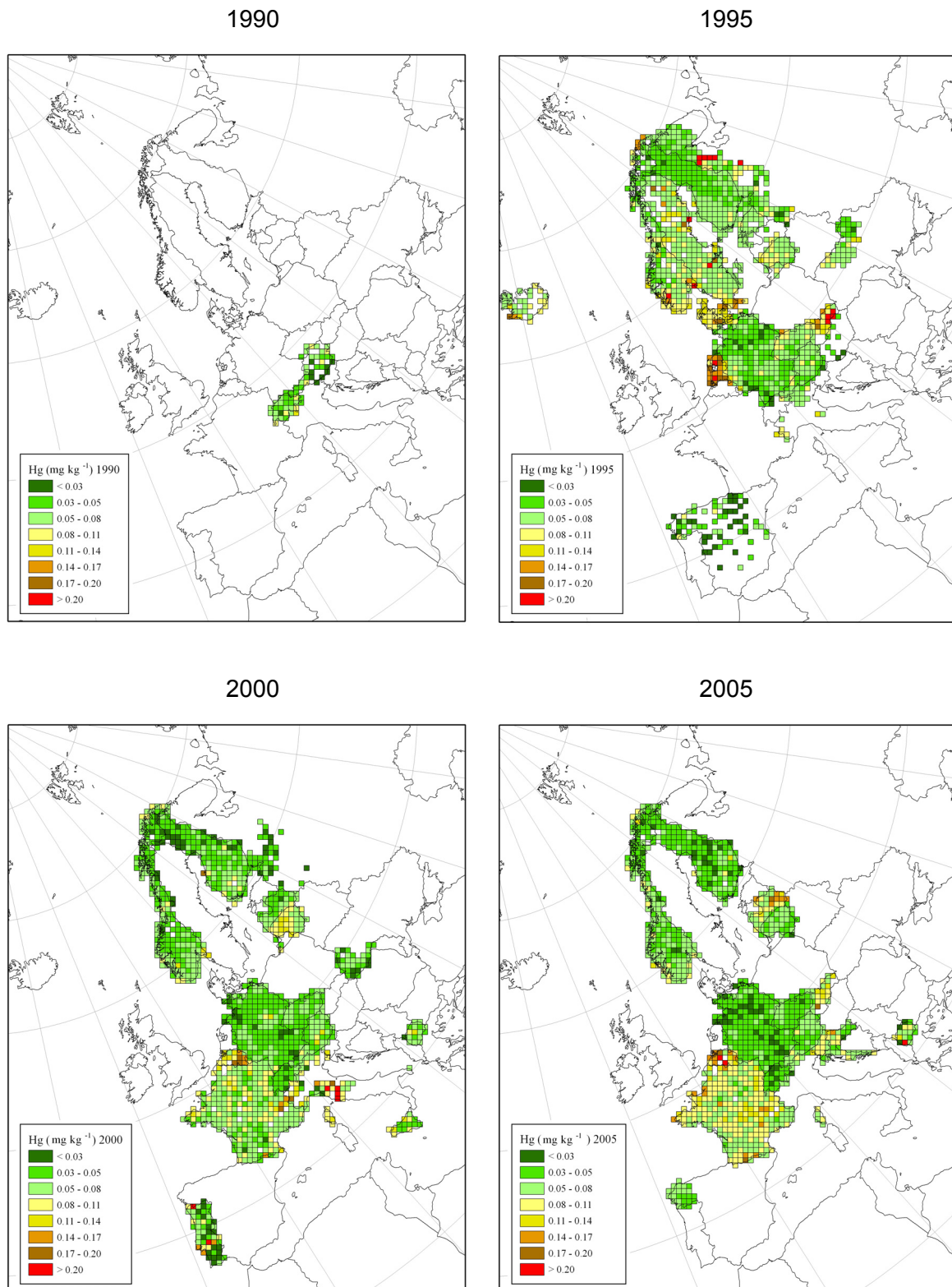
Figure 3.13. Mean concentration of mercury in mosses per EMEP grid square in 1990, 1995, 2000 and 2005.
